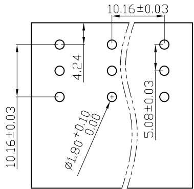
PCB LAYOUT
